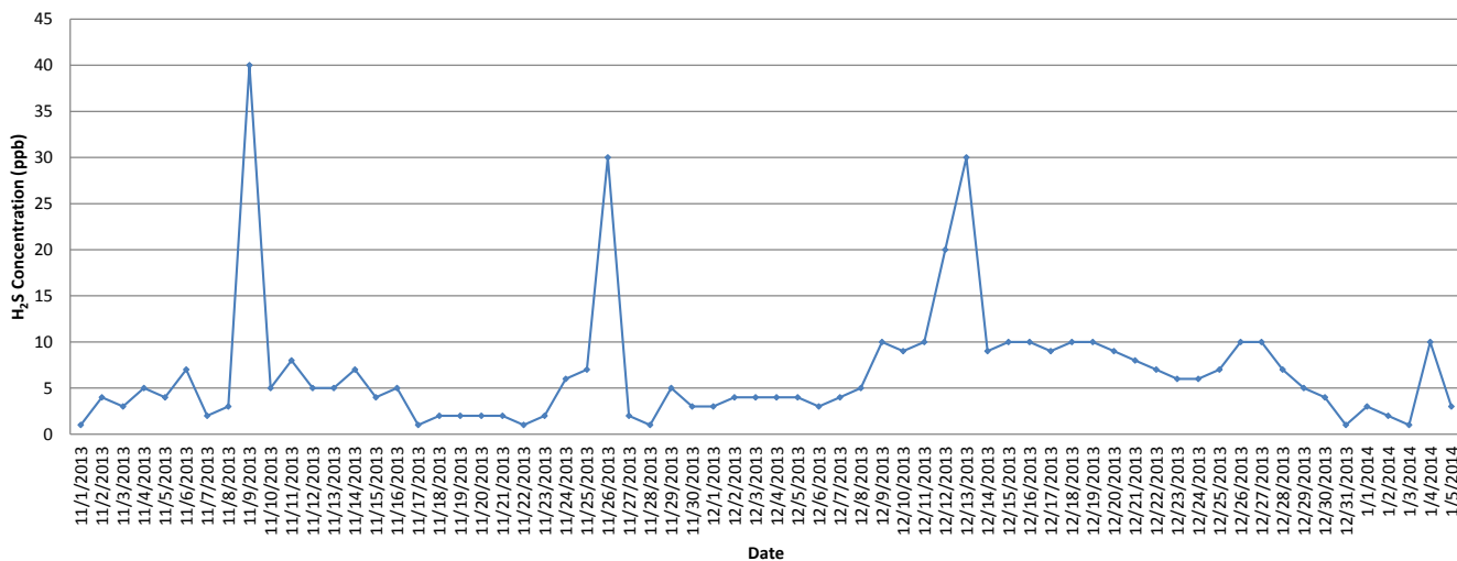
Daily Maximum Concentration of SO 2 from 11/1/13-1/5/14 @ ROX6
