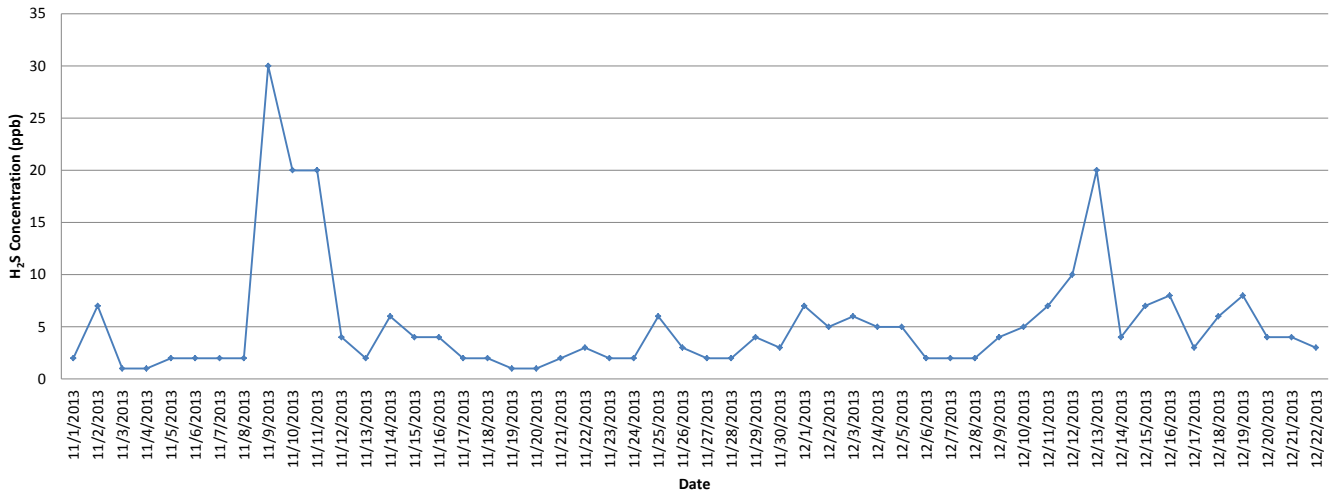
Daily Maximum Concentration of SO 2 from 11/1/13-12/22/13 @ ROX7
