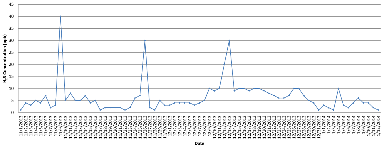
Daily Maximum Concentration of SO 2 from 11/1/13-1/12/14 @ ROX6
