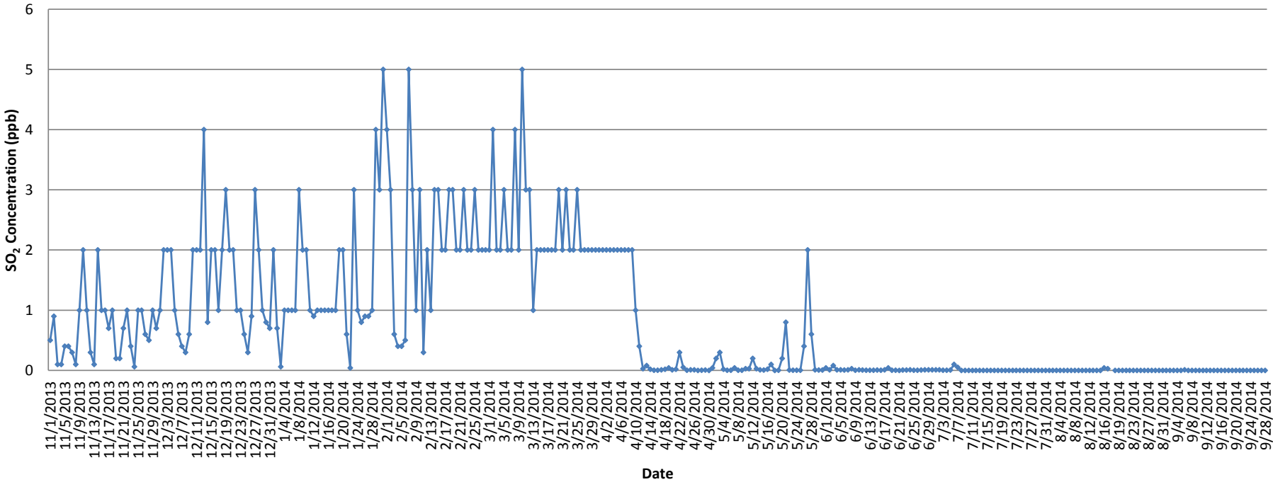
Daily Average Concentration of SO 2 @ ROX7
